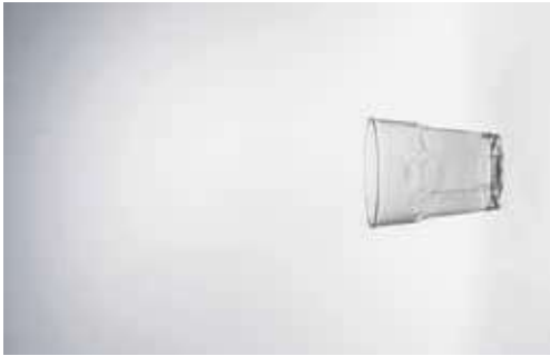
050828 OCTAGONAL GLASS 50 ml Ø 4.6 cm - h 5.3 cm Carton: 40 packs, 50 pcs/pack Pallet: 18 cartons/layer, 5 layers
