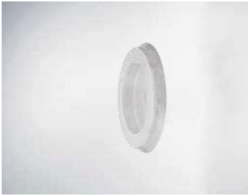
290115 LID K575 3.3 g - Ø 9.42 cm Carton: 16 packs, 50 pcs/pack Pallet: 4 cartons/layer, 3 layers
